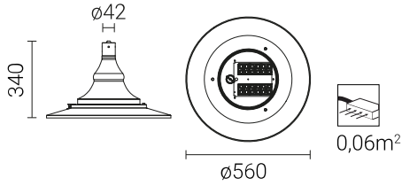
OW+ LED D4i WITH DIFFUSER
