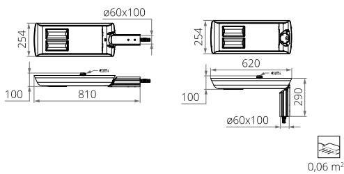
CUDDLE II LED ALFA REG D4i 96W, 120W, 144W, 196W
