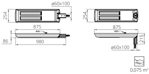
CUDDLE II LED ALFA REG D4i 48W, 60W, 72W
