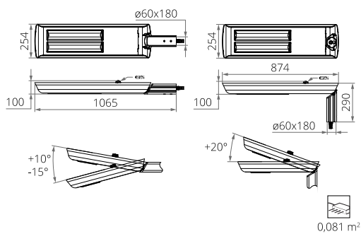
CUDDLE II LED ALFA REG D4i 96W, 120W, 144W, 196W
