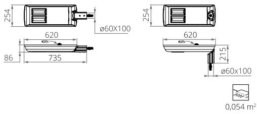
CUDDLE II LED REG D4i 96W, 120W, 144W, 196W
