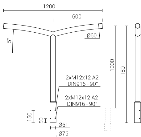
Code Symbol Number of arms Unit volume Effective projected area Luminaire mounting diameter Net weight 47250206/C... WR-5A/2/0,6/5 2 0.06 m³ 0.14 m² ø60 mm 4.5 kg
