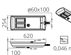
CUDDLE II LED D4i x2 47-72 W
