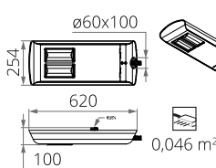
CUDDLE II LED D4i D 48-72 W
