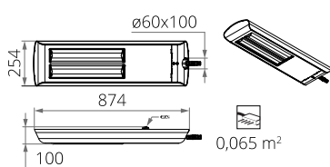
CUDDLE II LED D4i D 96-192 W
