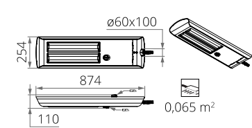
CUDDLE II LED D4i x2 96-192 W
