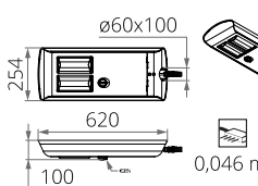
CUDDLE II LED D4i D 48-72 W
