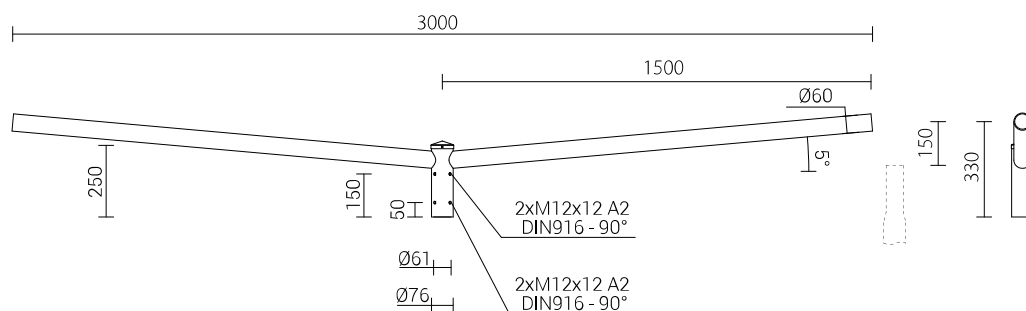
Code Symbol Number of arms Unit volume Effective projected area Luminaire mounting diameter Net weight 472042159/C... WR-4/2/1,5/5 ZP 2 0.48 m³ 0.196 m² ø60 mm 5.9 kg
