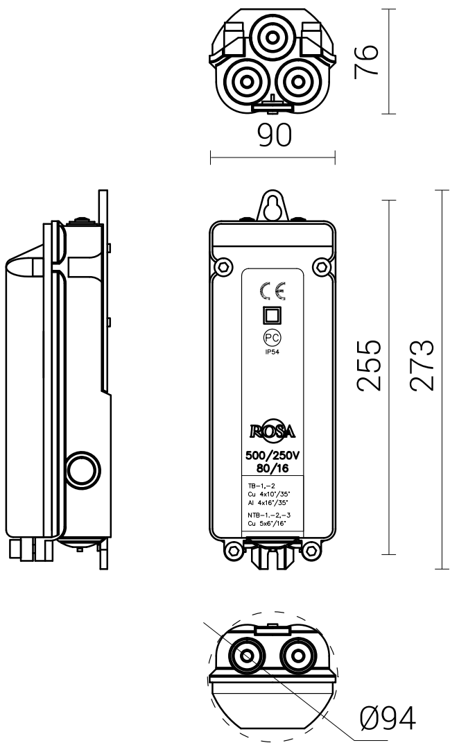
Fuse-link D01
