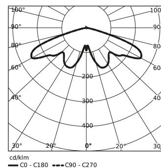
VS - RING LED 72 W
