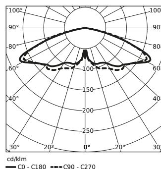
VS - RING LED 24 - 48 W
