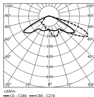
T4 - RING LED 72 W
