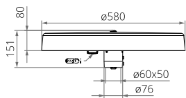
RING 3 LED D4i 'A'
