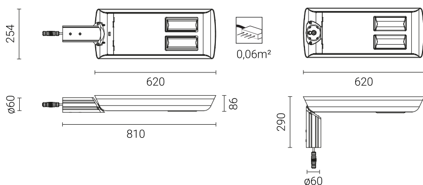
CUDDLE II LED REG 48W, 60W, 72W
