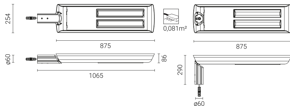
CUDDLE II LED REG 96W, 120W, 144W, 192W
