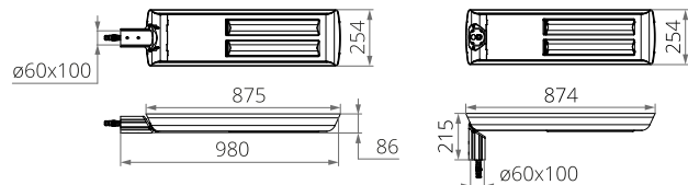
CUDDLE II LED ALFA REG 48W, 60W, 72W
