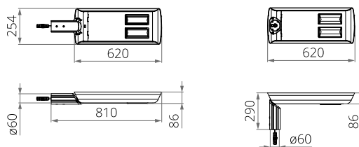
CUDDLE II LED ALFA REG 96W, 120W, 144W, 192W
