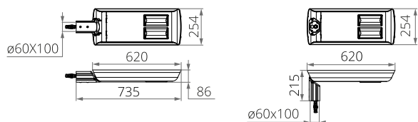
CUDDLE II LED REG 96W, 120W, 144W, 196W
