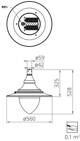
OPTIONAL VERSION OW+ LED D4i WITH DIFFUSER
