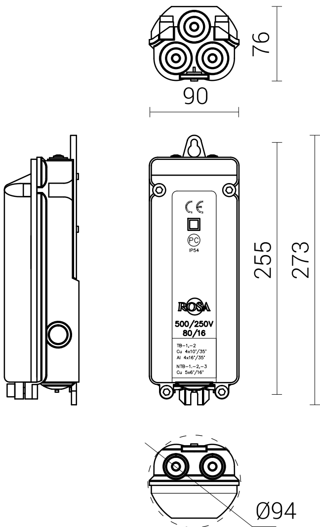
Fuse-link D01
