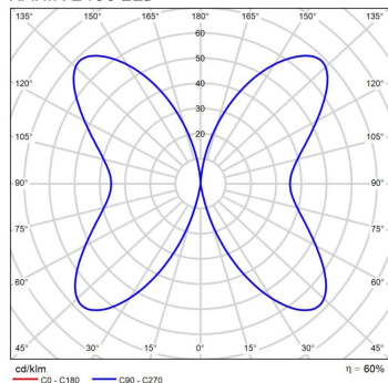
KARIN 2400 LED
