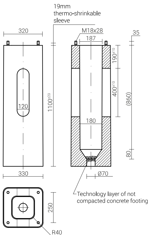
Code Symbol Fasteners Bolt spacing E [mm] Thread length C [mm] Height of threaded anchor ending C [mm] Dimension AxBxH [mm] Net weight 311160 B-60 4008 250 28 35 320x330x1100 176 kg
