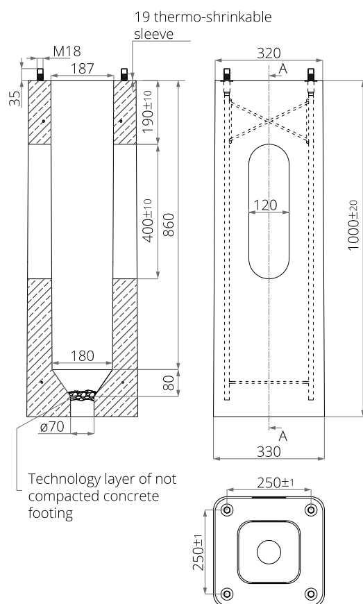
Code Symbol Fasteners Bolt spacing E [mm] Thread length C [mm] Height of threaded anchor ending C [mm] Dimension AxBxH [mm] Net weight 311160 B-60 4008 250 28 35 320x330x1000 176 kg
