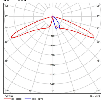
CUT-1 LED
