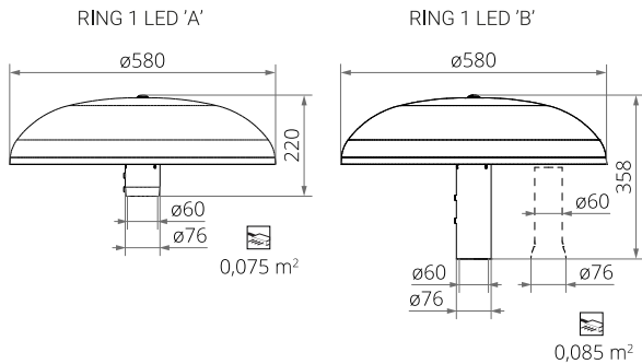
T4 - RING LED 24 - 48 W
