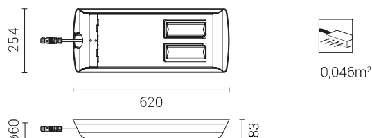
CUDDLE II LED 48W, 60W, 72W
