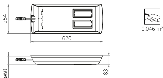
CUDDLE II LED 96W, 120W, 144W, 192W
