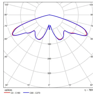
VS - RING LED D4i 72 W
