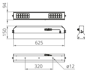
ISKRA LED LB 80
