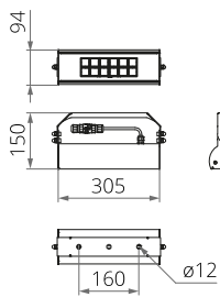
ISKRA LED LB 36
